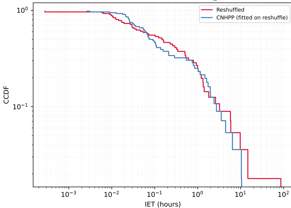
User 802665649 - Reshuffled vs CNHPP A_{\text{fit}}=0.5358
